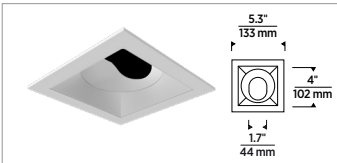
SQUARE FLANGED
