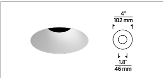
ROUND FLANGELESS
