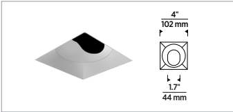
SQUARE FLANGELESS
