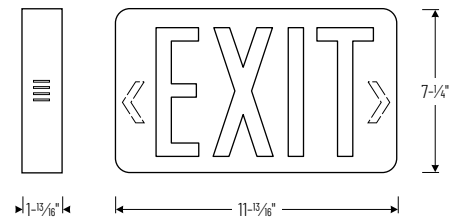
NX-603D-LED/B Dual Color / Black Housing
