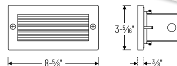
NSW-841/SC Louver Face Plate
