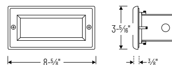
NSW-842/SC Lensed Face Plate
