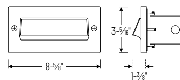
NSW-843/SC Shroud Face Plate
