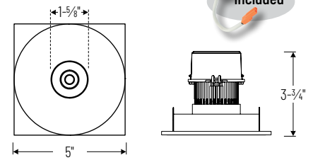
NPR-4SNB Square Bullnose Non-Adjustable
