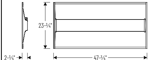
NPTCBSW-24/SCW 2' x 4' LED Troffer
