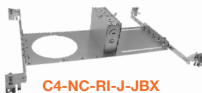
C4-NC-RI-J-JBX 17" W x 6.5" D x 3.5" H 5" Hole 14" Min. Extend 25" Max. Extend (Assembly Required)
