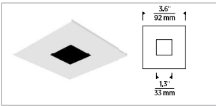
SQUARE FLAT
