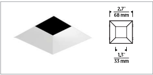
SQUARE BEVEL
