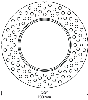
ROUND DIE-CAST
