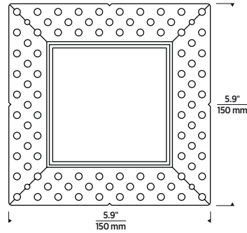
SQUARE DIE-CAST
